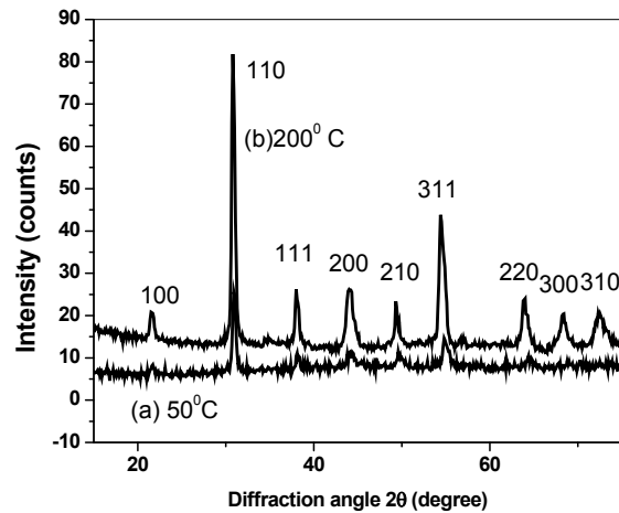
Fig. 2. XRD diffraction pattern of the PZT-5A at: (a) 50°C and (b) 200°C
