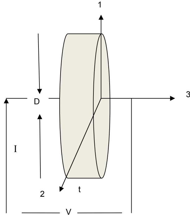
Fig. 1. PZT disc under compression force acting on direction 3
