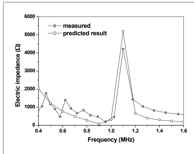
Fig. 3. electrical magnitude spectrum for the disk of PZT-5A
