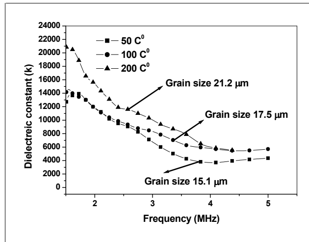
Fig. 4a. Change of dielectric constant with frequency of PZT-5A
