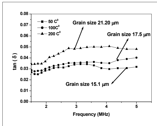
Fig. 4b. Change of dielectric loss with a frequency of PZT-5A
