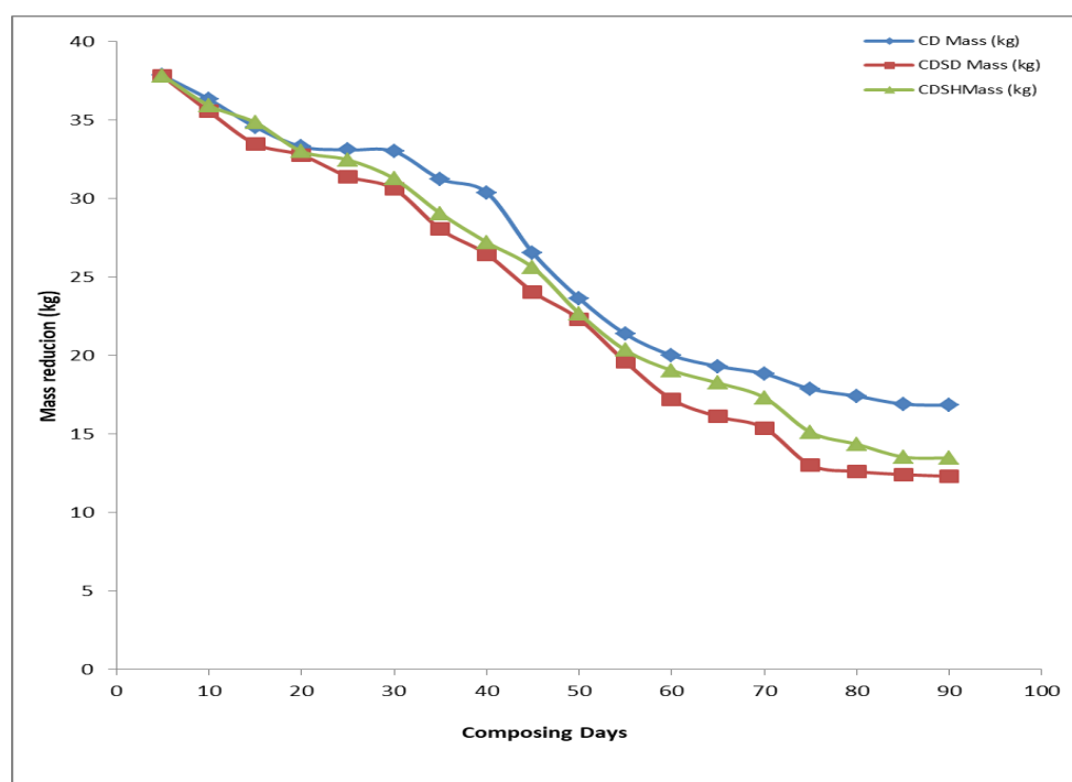
Fig. 6. Weight reduction in composting mixtures
