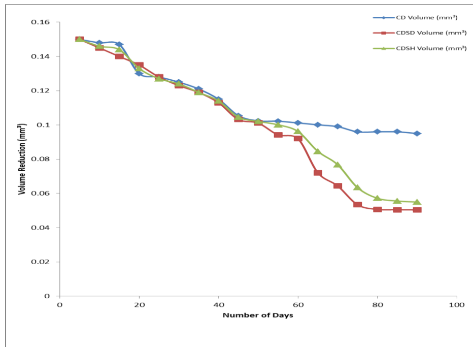
Fig. 5. Volume reduction in composting mixtures
