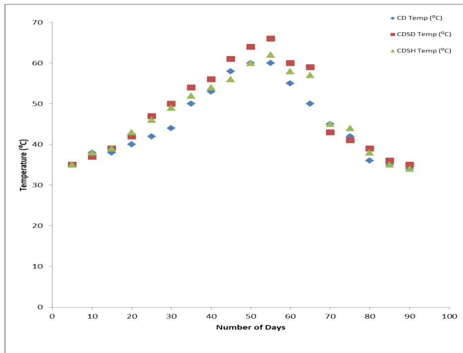
Fig. 4. Temperature variations of composting mixtures
