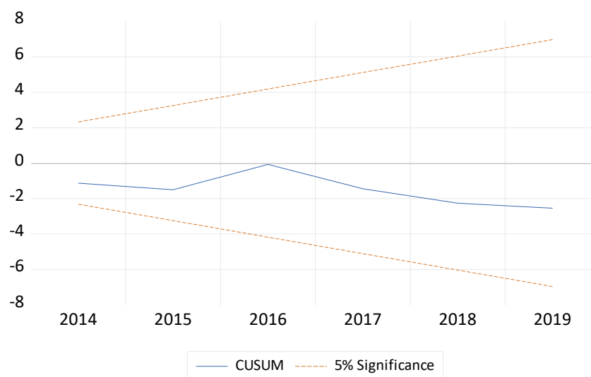
Fig. 1. Plot of cumulative sum (CUSUM) of recursive residuals
